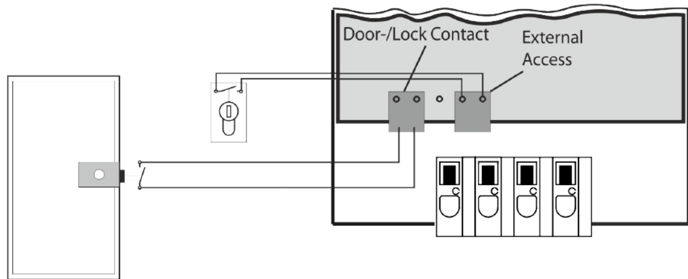
Figure 3: Connection of Door-/Lock Contact and External Access
